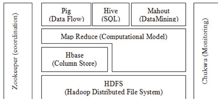
Fig 2: Architecture of Hadoop
